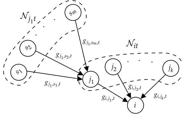
FIGURE 2. Second-degree innovation connections among firms
