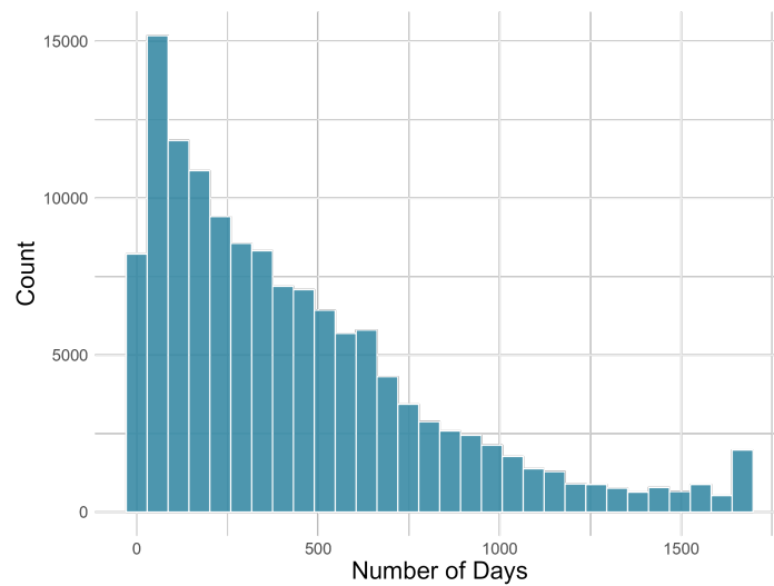
FIGURE A3. Frequency of unique pairs of firms appearing in our final dataset
