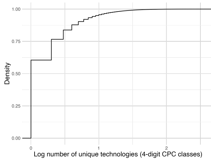
FIGURE A2. Distribution of the number of distinct technologies cited by a firm
