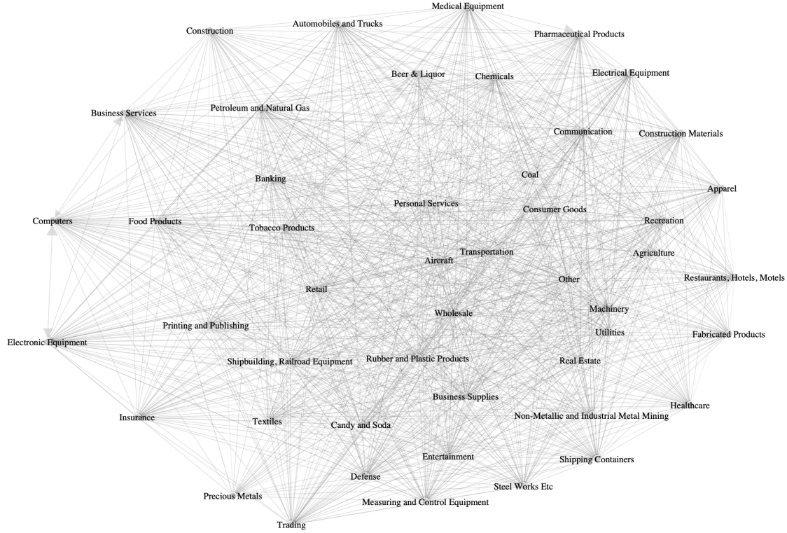
FIGURE A1. Directed innovation network across industries
