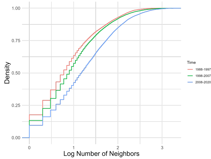
FIGURE A5. Neighborhood size
